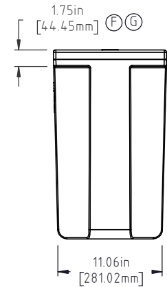
DETAIL A SCALE 1 : 6
