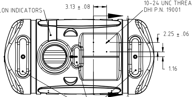
FLATS FOR PICKUP/RETURN LINE PLACEMENT
