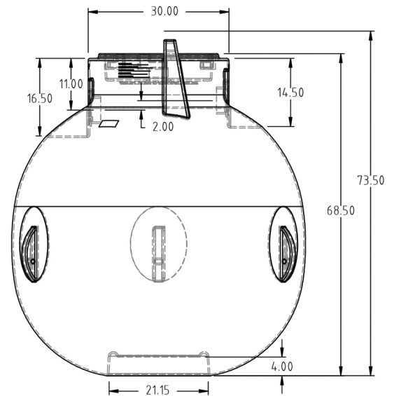
AST-0500-1R Dimensions: 63" x 74" Weight: 197 lbs Tank UPC: 768570443442
