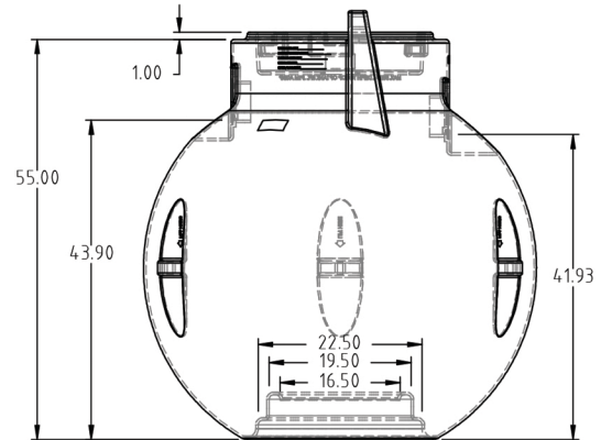
AST-0300-1R Dimensions: 54" x 56" Weight: 137 lbs Tank UPC: 768570443435
