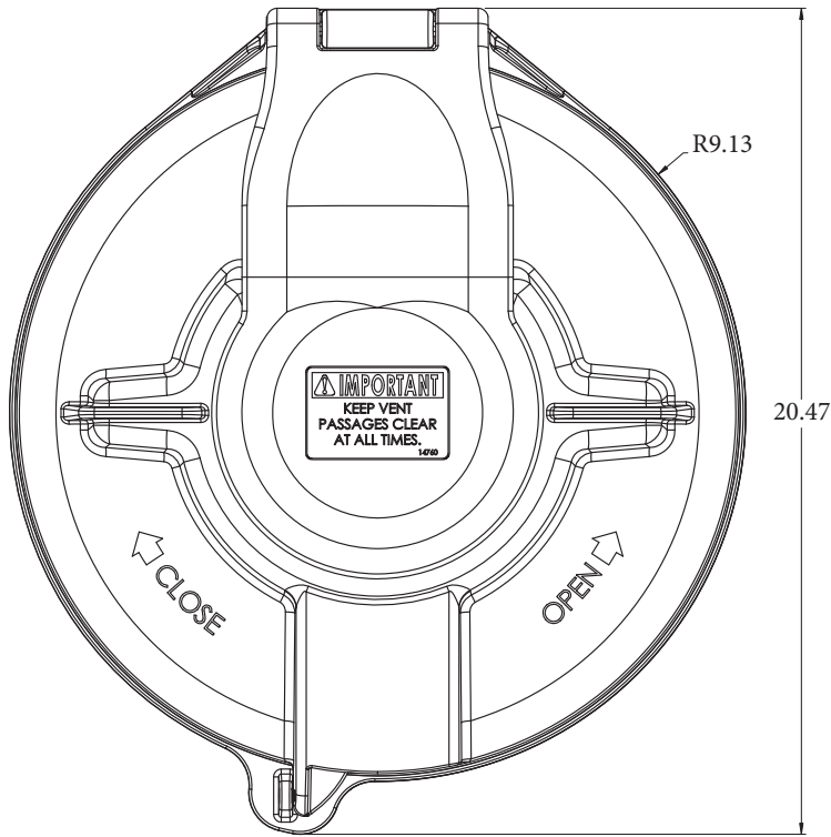
16" Hinged Lid Assembly Vented Product Number: 14761
