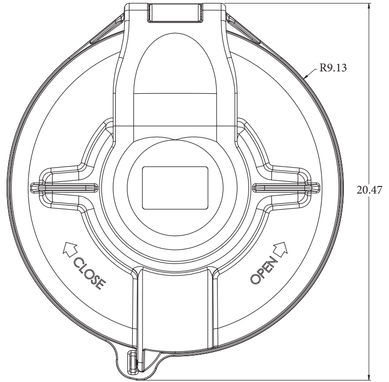
16" Hinged Lid Assembly Non-Vented Product Number: 14762
