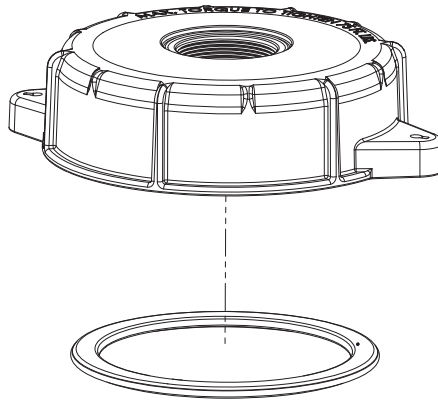
6" Cap - 2" NPS Thread and Gasket Assembly Santoprene or Viton
