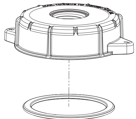
6" Cap - 2-2.5" Buttress Thread and Gasket Assembly Santoprene or Viton
