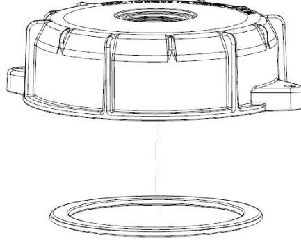
9" Cap - 2" FPT Thread and Gasket Assembly Santoprene or Viton
