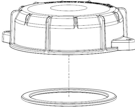
9" Cap without Port and Gasket Assembly Santoprene or Viton
