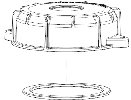
9" Cap - 2.5-5 Buttress Thread and Gasket Assembly Santoprene or Viton
