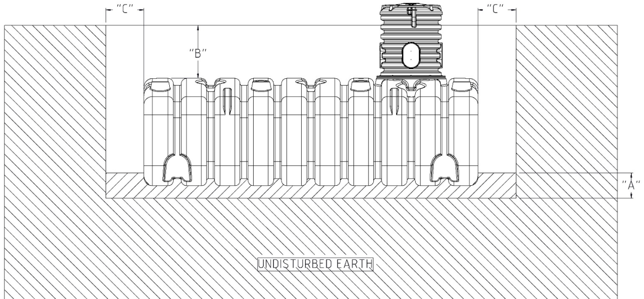
FIGURE 1: SITE EXCAVATION
