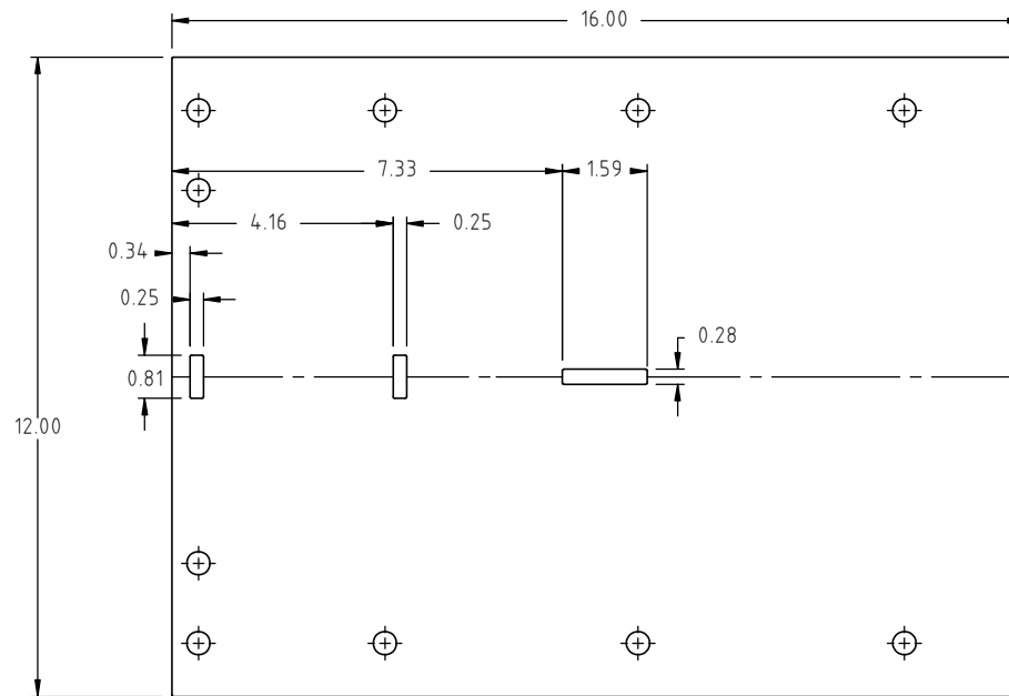
FLAT PATTERN
