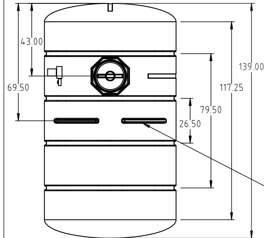
FM1610-78C CENTER DRAIN SUMP
