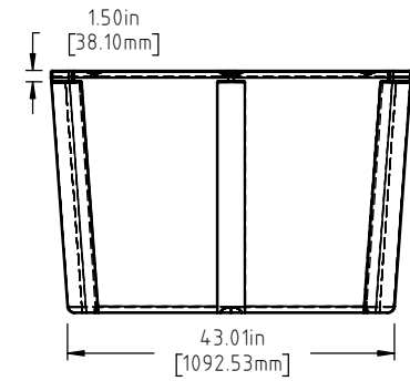
DETAIL A SCALE 1: 6
